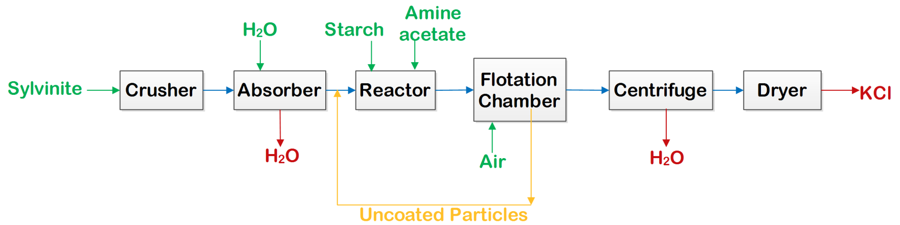
Figure: Manufacturing of Potassium Chloride by Flotation Process
